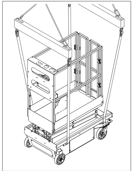
FIGURE 9: Example Sling/Lifting
