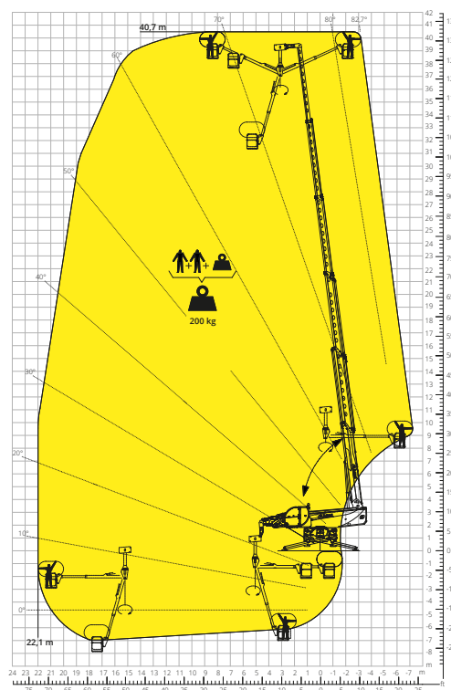
Load chart with OVER-UNDER PLATFORM - NEGATIVE ATT - 01 - 024
